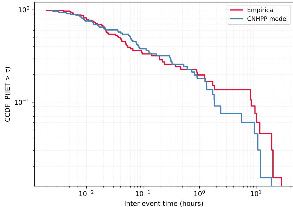
User 10749503 - Empirical vs CNHPP model
